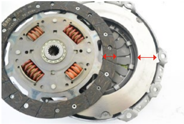
Example of a friction disc with a Larger ID than the Pressure Plate friction surface.
