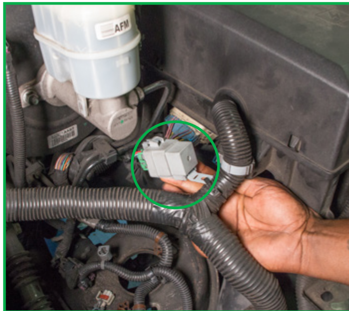
GM SUVS/TRUCKS (GMT8XX/9XX/K2XX) Relay located on left side of engine compartment near the Underhood Fuse Block
