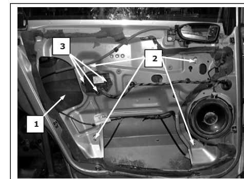
Porta lato sinistro, Portière arrière gauche, Left rear door, Puerta lado izquierdo, Hinten links Tür, Porta traseira esquerda, Sol arka kapi, νότρο οπισθία αριστερή
