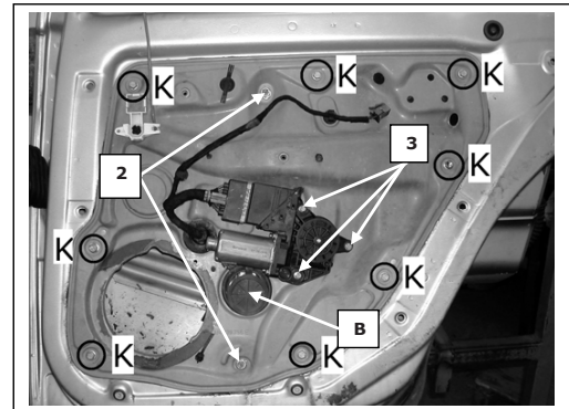
Porta lato destro, Portière arrière droite, Right rear door, Puerta lado derecho, Hinten rechte Tür, Porta traseira direita, Sağ arka kapi, πόρτα οπίσθια δεξιά
