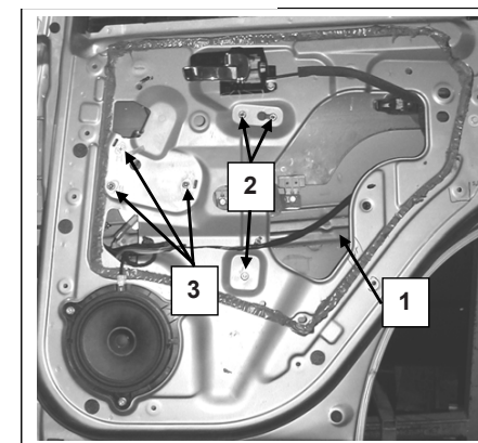
Porta lato destro, Portière arrière droite, Right rear door, Puerta lado derecho, Hinten rechte Tür, Porta traseira direita, Sag arka kapi, πόρτα οπίσθια δεξιά
