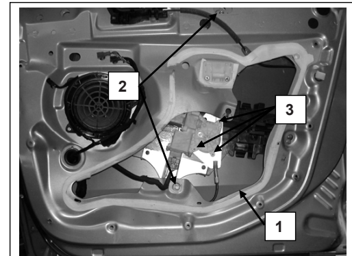
Porta lato destro, Portière avant droite, Right front door, Puerta lado derecho, Vorne rechte Tür, Porta frente dijeta, Sag on kapi, πόρτα εμπρός/α δεξιά
