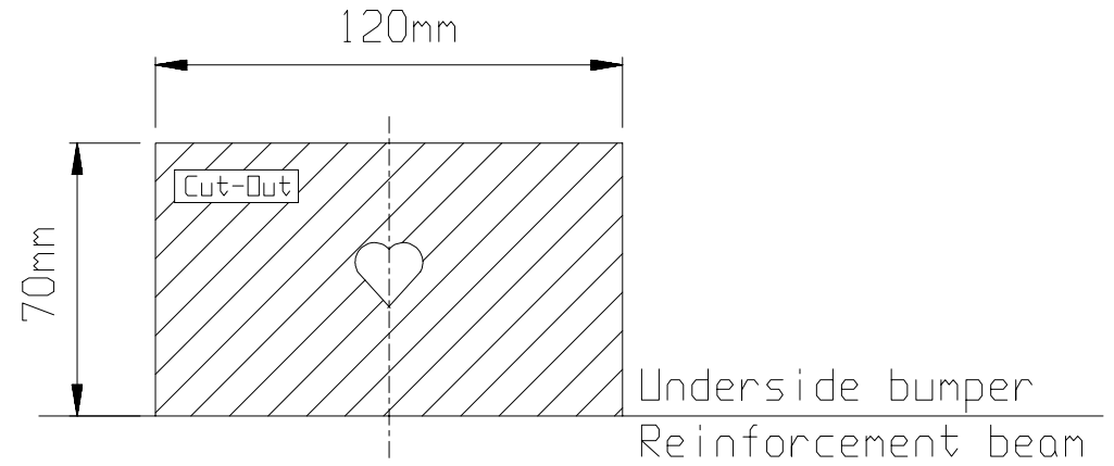
Detail 2
